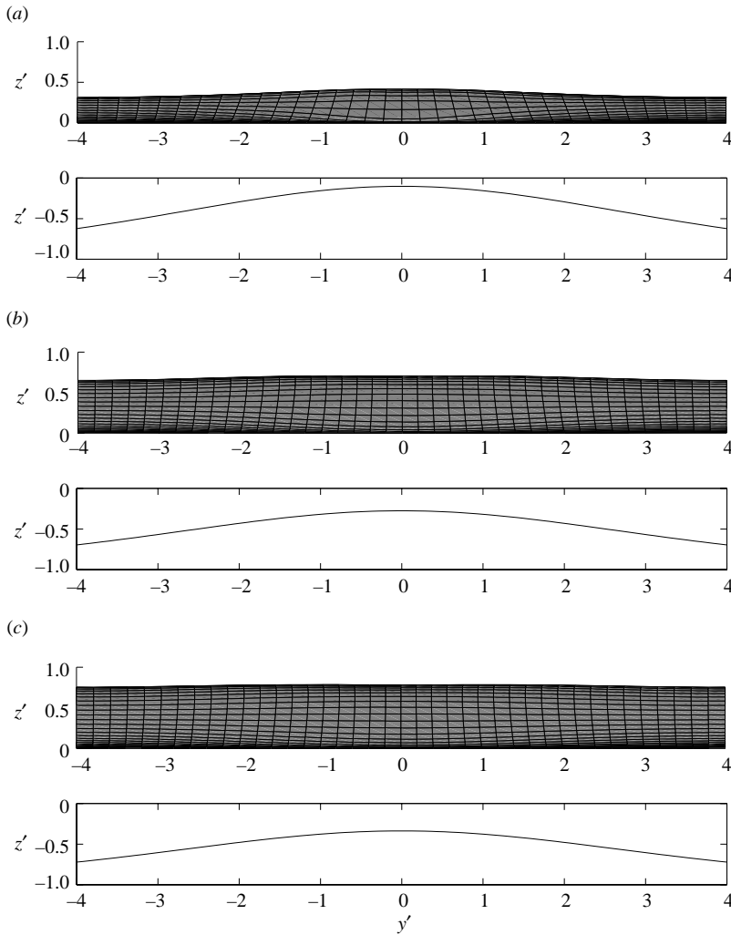
FIGURE 24. k = 0.25 . Front view of wave (upper panel) and bottom (lower panel) profiles at the breaking point for (a) H'_0 = 0.3 ( t'_B = 10.881 , x'_B = 18.691 ), (b) H'_0 = 0.6 ( t'_B = 7.890 , x'_B = 16.093 ) and (c) H'_0 = 0.7 ( t'_B = 7.250 , x'_B = 15.164 ).
